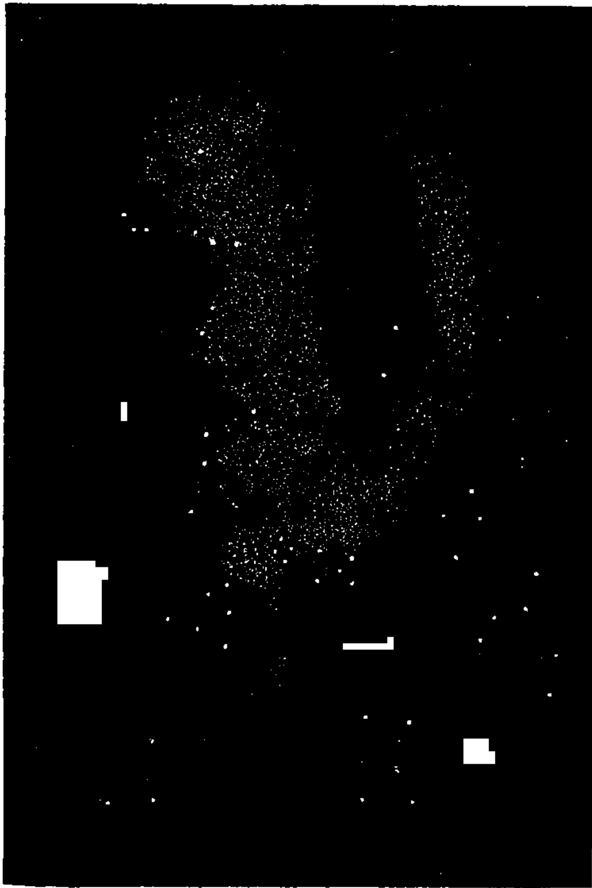
FROM THE GREAT NEBULA IN ORION.
