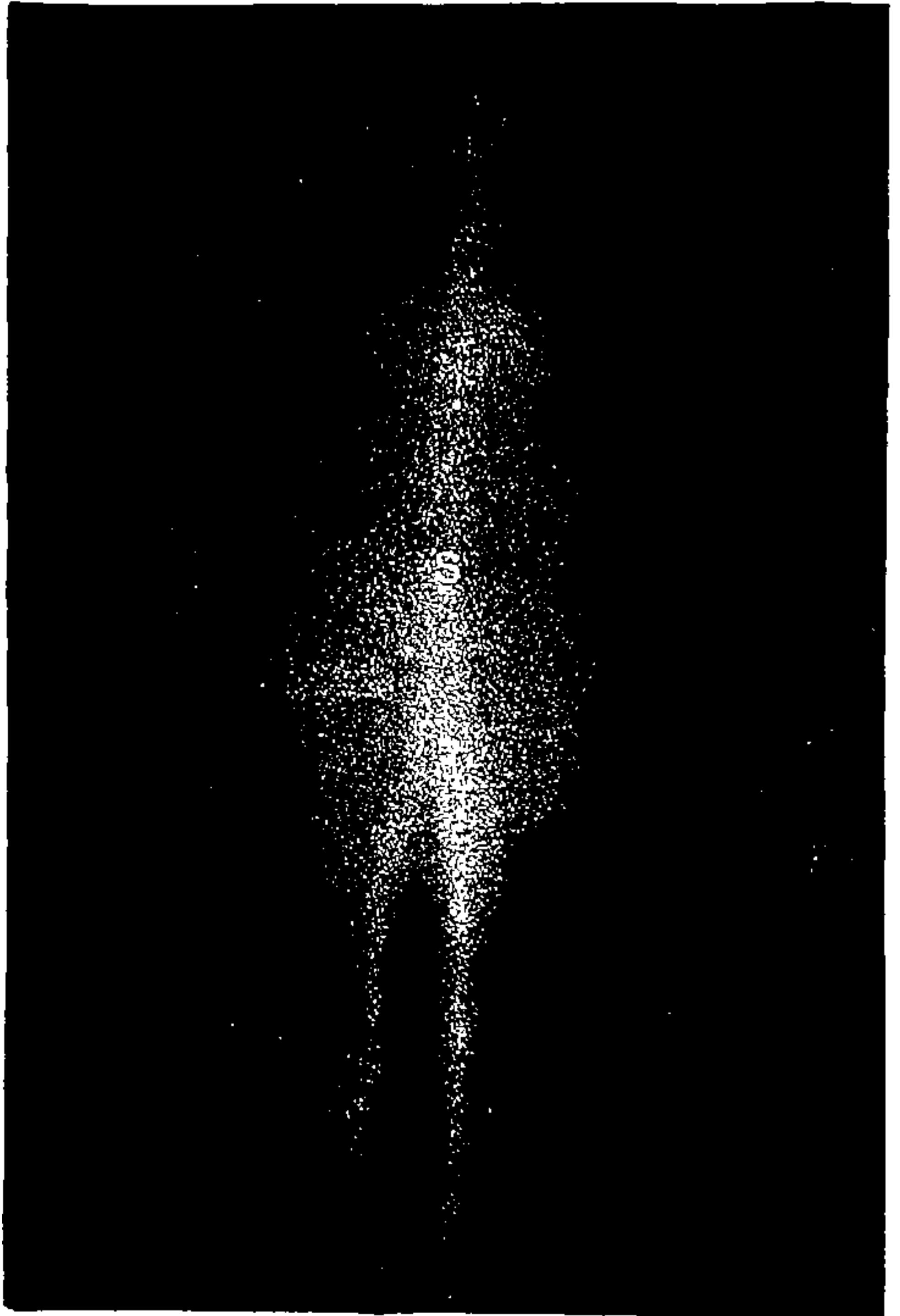
THE GALAXY ACCORDING TO HERSCHEL.
