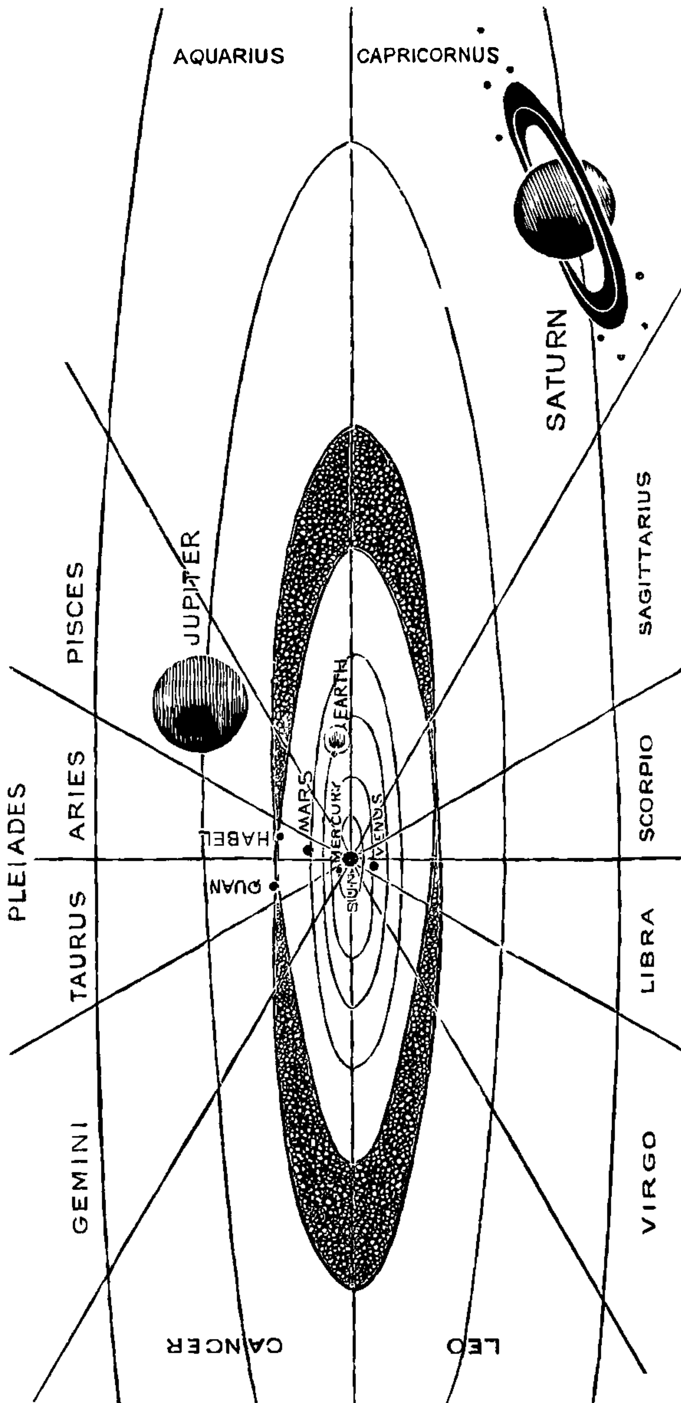
THE SOLAR SYSTEM, WITH THE BELT OF ASTEROIDS, ACCORDING TO TISSERAND.
